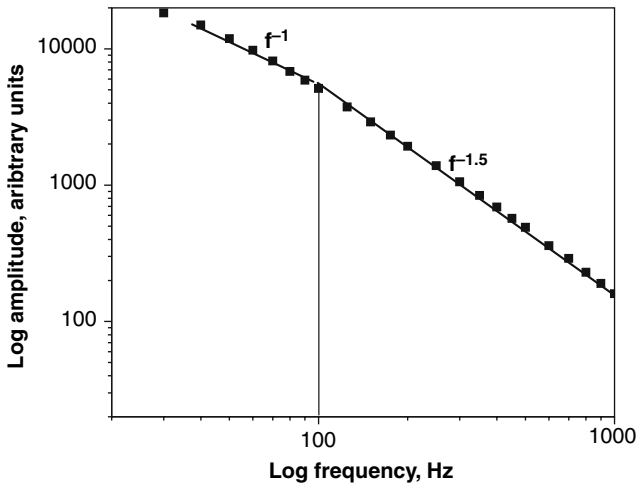
Fig. 3. Log-Log plot of PA amplitude for \text{LaPO}_4 sintered at 800^\circ\text{C} .
